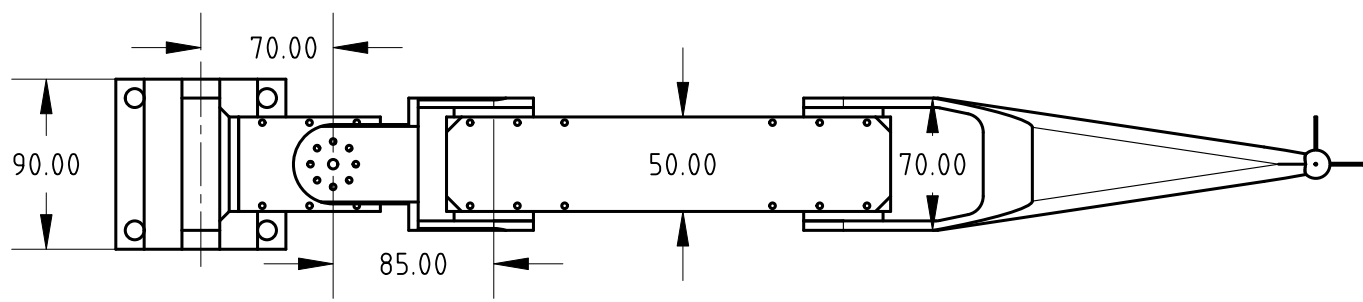
1:4 Top view
