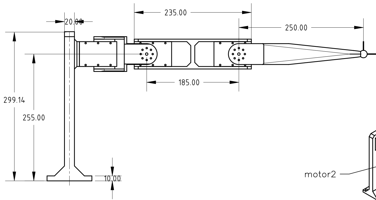
1:4 Front view
